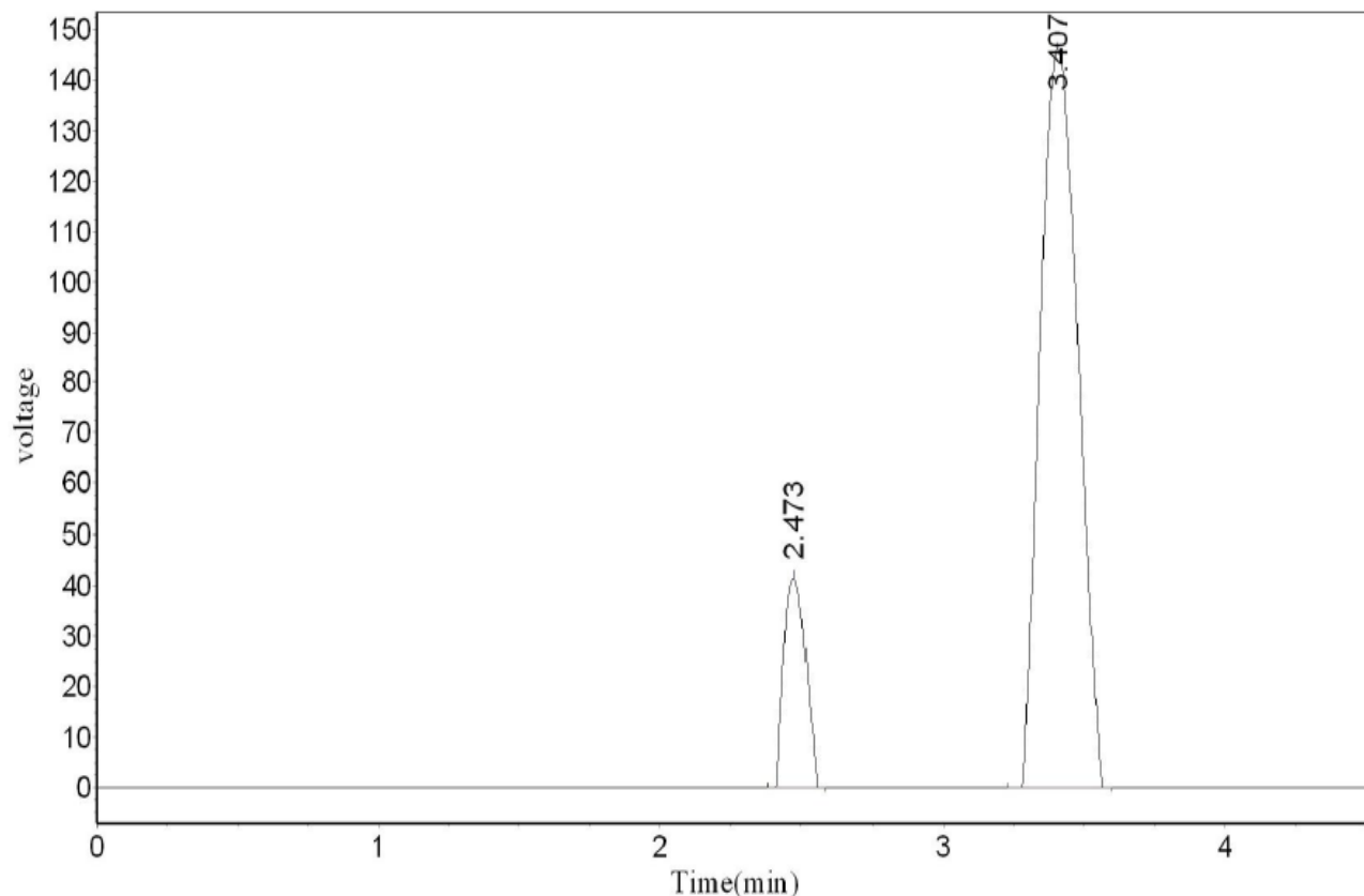
Figure 1.1 Optimized chromatogram
