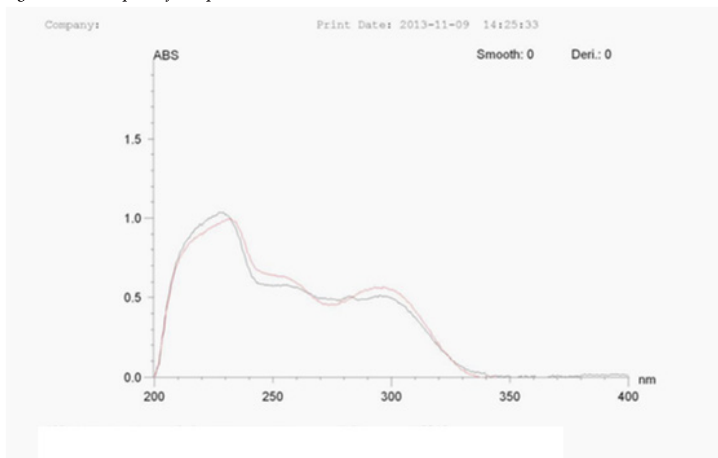
Figure-1. Isobestic point of Metoprolol And Telmisartan.
