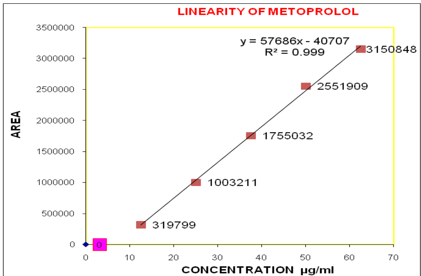
Fig 2: LINEARITY GRAPHS OF METOPROLOL AND TELMISARTAN
